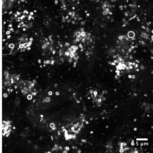
Figure 3: mEGFP-tagged LAMP1 localization in an hiPSC colony. Image is a single slice from a 3D spinning disk confocal z-stack of a live hiPSC colony in the top half of the cells.
