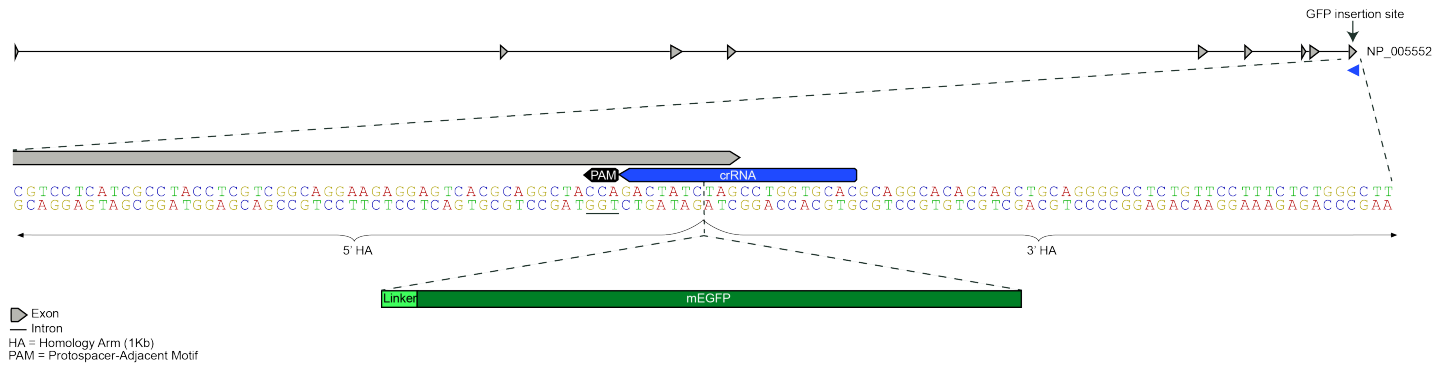
Figure 1: Top: LAMP1 locus; Bottom: Zoom in on mEGFP insertion site at LAMP1 C-terminal exon
