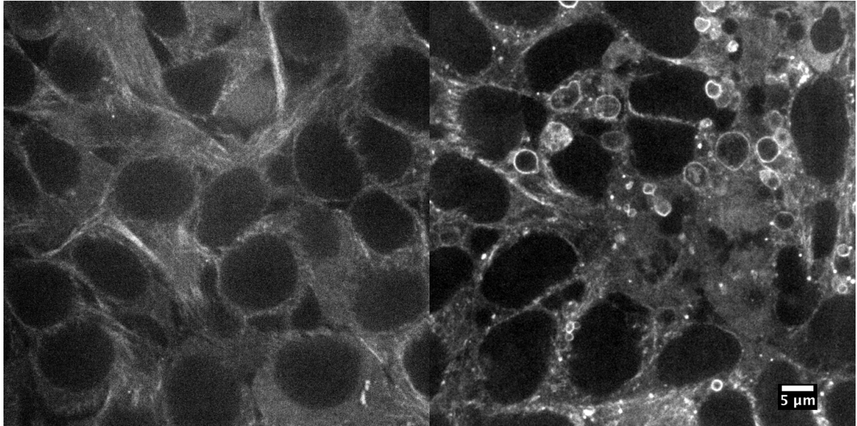
Figure 3: mEGFP-tagged autophagy-related protein LC3 B localization in an hiPSC colony. Image is a single slice of a 3D spinning disk confocal z-stack of a live hiPSC colony in the bottom half of the cells. Both untreated cells (left panel) and cells treated for 24 hours with 800nM leupeptin to visualize autophagosomes (right panel) are shown.
