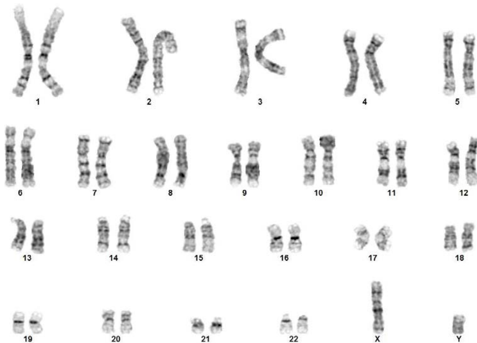
Figure 5. G-banding karyogram
