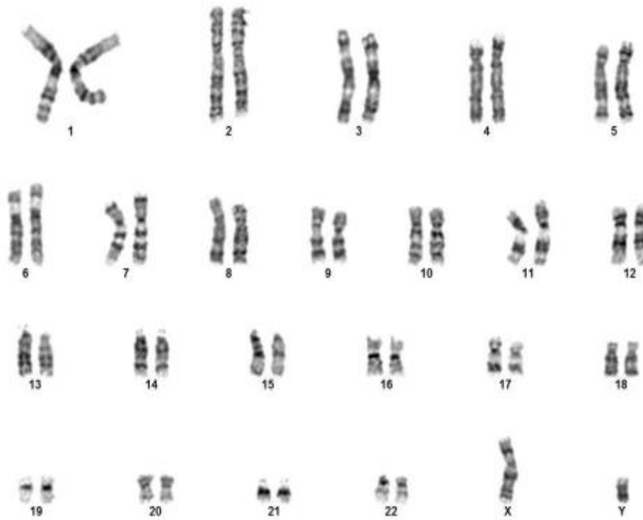
Figure 5. G-banding karyogram
