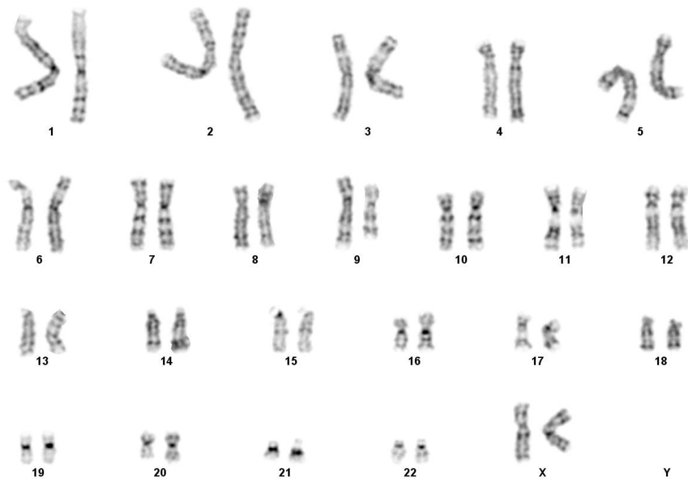
Figure 5. G-banding karyogram
